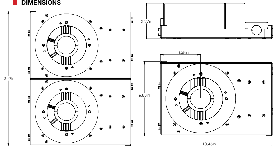
Modular Conjoined Configuration for 16 " Stud Separation
