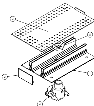
Beginning Module Length: 5 inches Purpose: To be attached at the beginning of ZENLITE® channel by means of two T-shape connectors Sub-Components: 1. 4 in Channel 2. End Cap 3. Channel Cover 4. BX Cable Connector 5. BX Connector Nut Part #: ZNLT-BGNM-NC1-5/8
