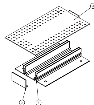
End Module Length: 5 inches Purpose: To be attached at the beginning of ZENLITE® channel by means of two T-shape connectors Sub-Components: 1. 4 in Channel 2. End Cap 3. Channel Cover Part #: ZNLT-ENDM-NC1-5/8
